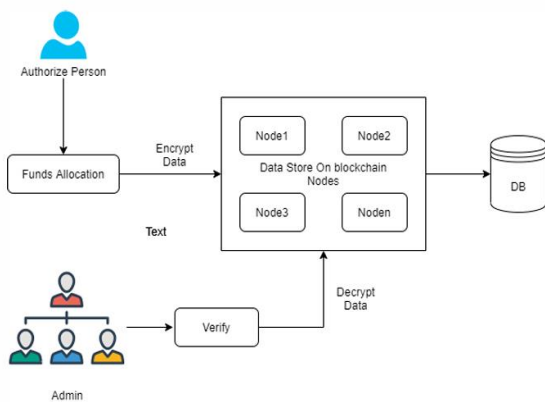
Fig. 1: Architecture Diagram
