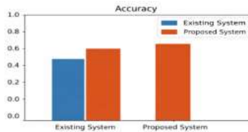
FIG 2.BAR GRAPH
