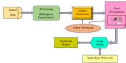
FIG 1.SYSTEM ARCHITECTURE
